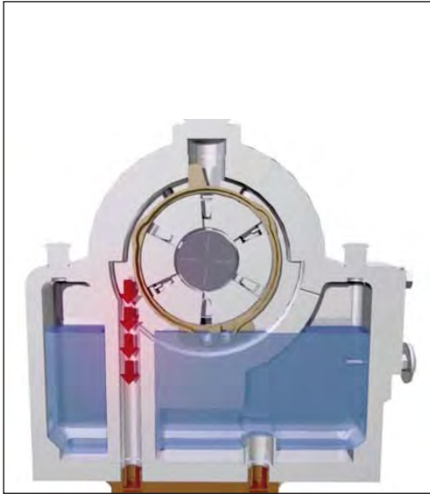
Hot oil from the thrust bearings returns to the heat exchanger through a standpipe.
