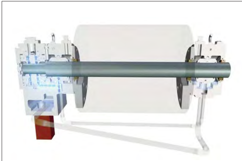
As pressurized oil is supplied to the integral journal in the CH unit, it also travels to the journal in the remote C bearing. Hot oil returns to the reservoir by customer-supplied piping.
